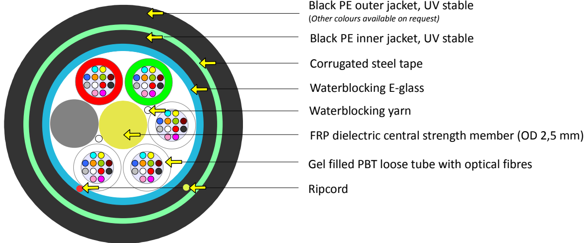
The picture represents a cable with 60 fibres.
