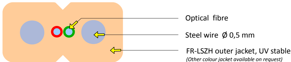
The picture represents a cable with 2 fibres.
